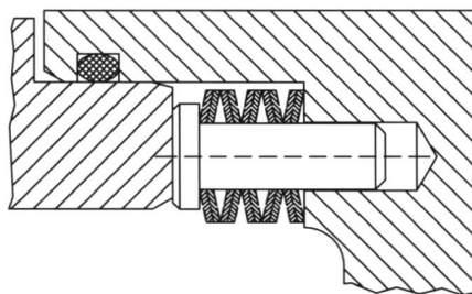
Contact pressure system up to DN 100 and above
