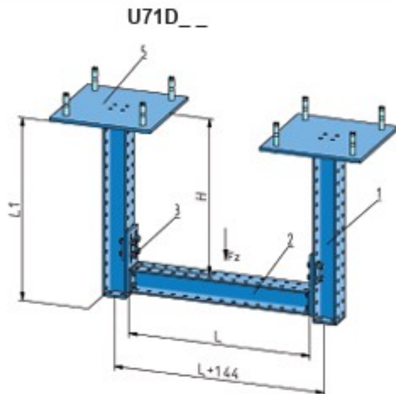
Bridge U71D_ _ (Plugplate)
