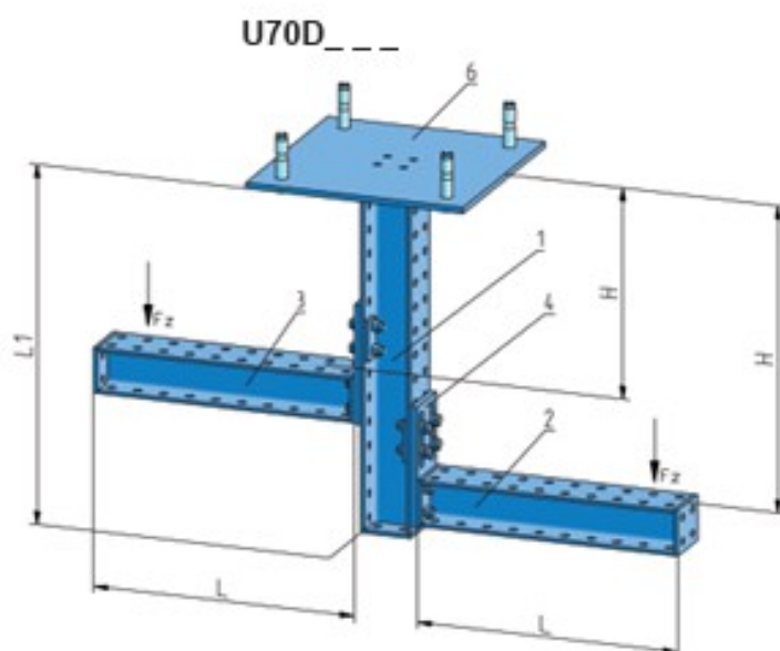
Scaffold U70D_ _ _ (Plugplate)
