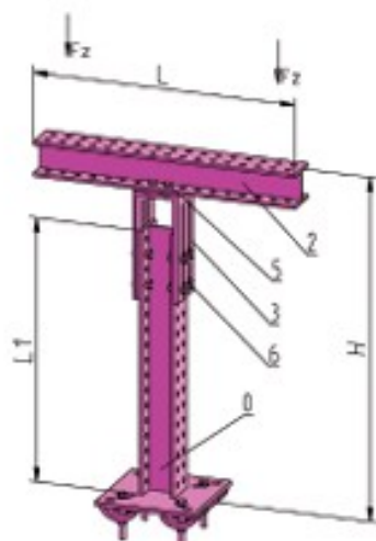
T-Support UL64K__0 (Connection section 80-120)
